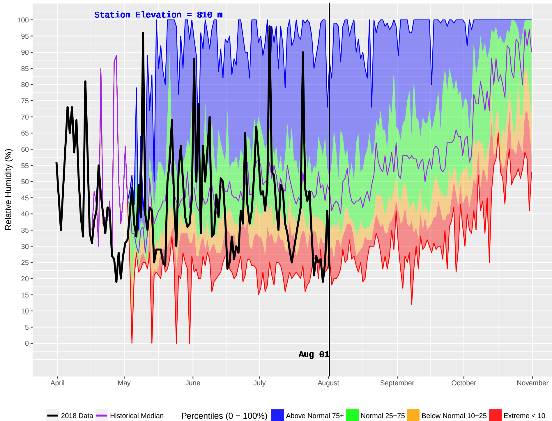
MCBRIDE LAKE (180) : Historical (1990–2016) and Current (2018) Daily Relative Humidity
