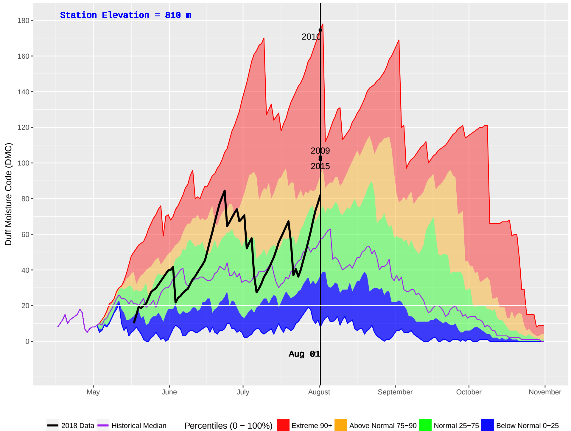
MCBRIDE LAKE (180) : Historical (1990–2016) and Current (2018) Daily Duff Moisture Code (DMC)
