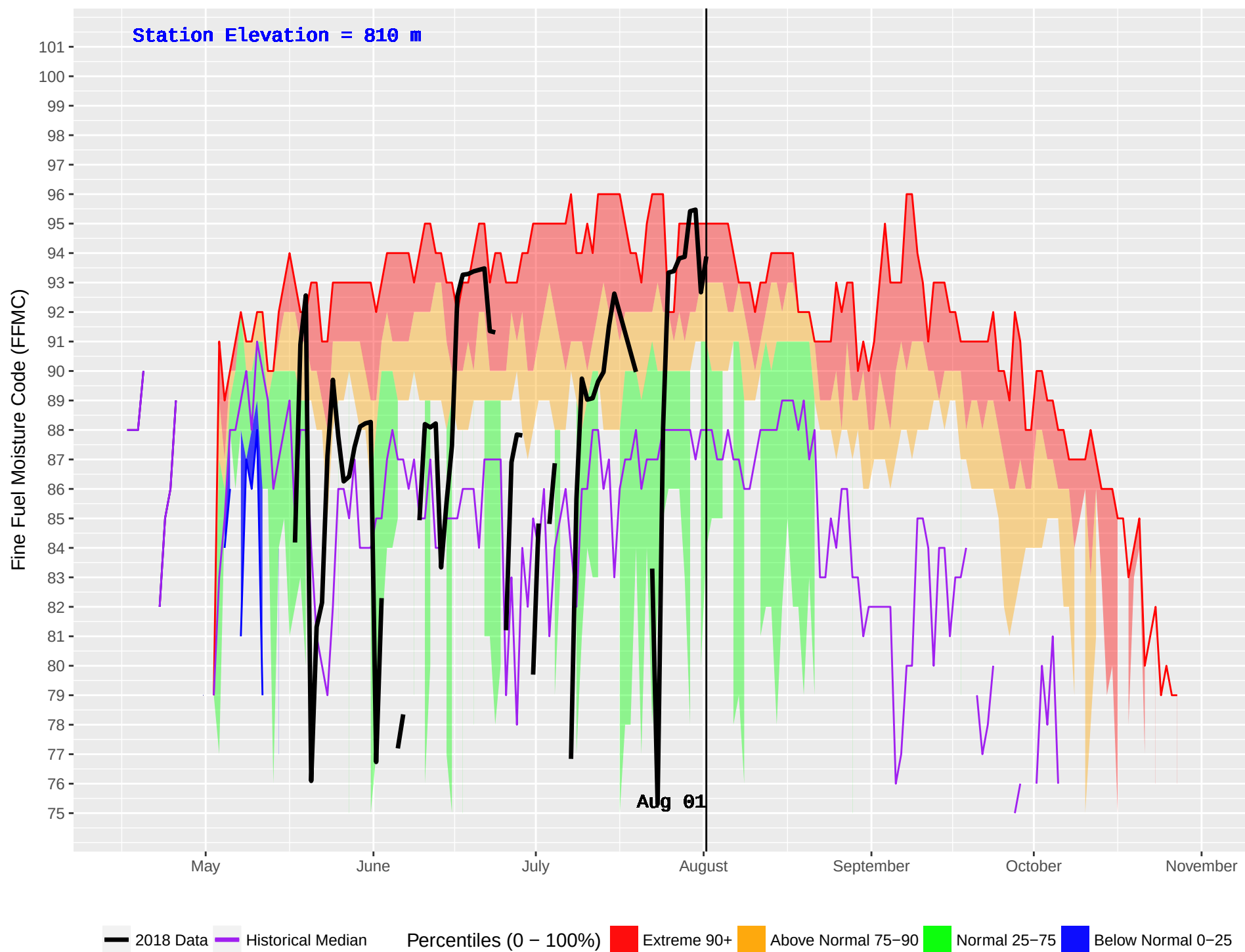
MCBRIDE LAKE (180) : Historical (1990–2016) and Current (2018) Daily Fine Fuel Moisture Code (FFMC)
