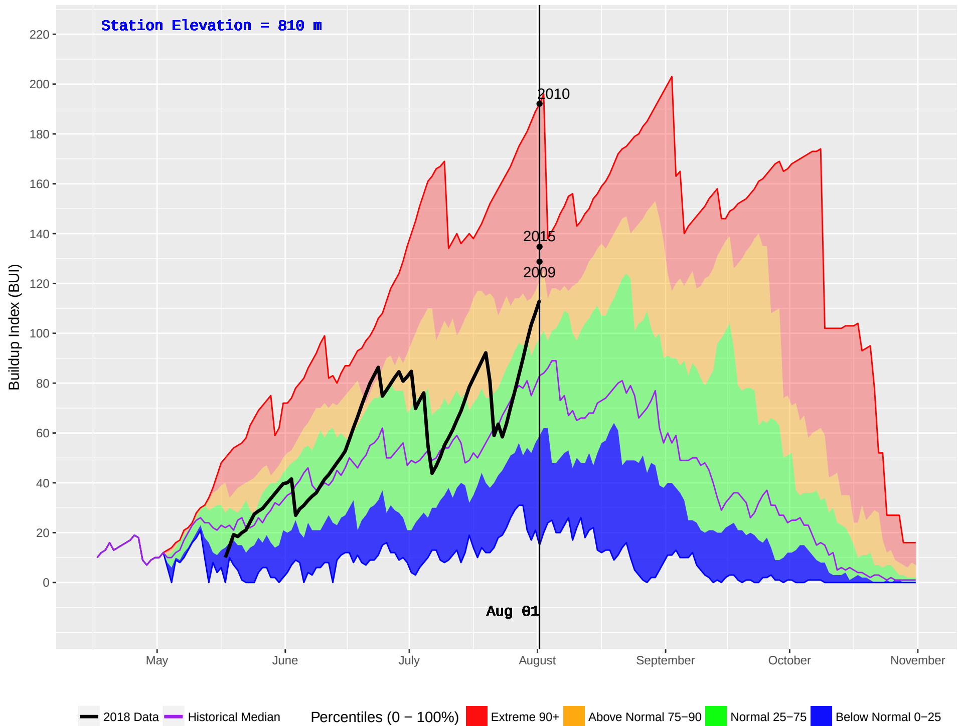
MCBRIDE LAKE (180) : Historical (1990–2016) and Current (2018) Daily Buildup Index (BUI)
