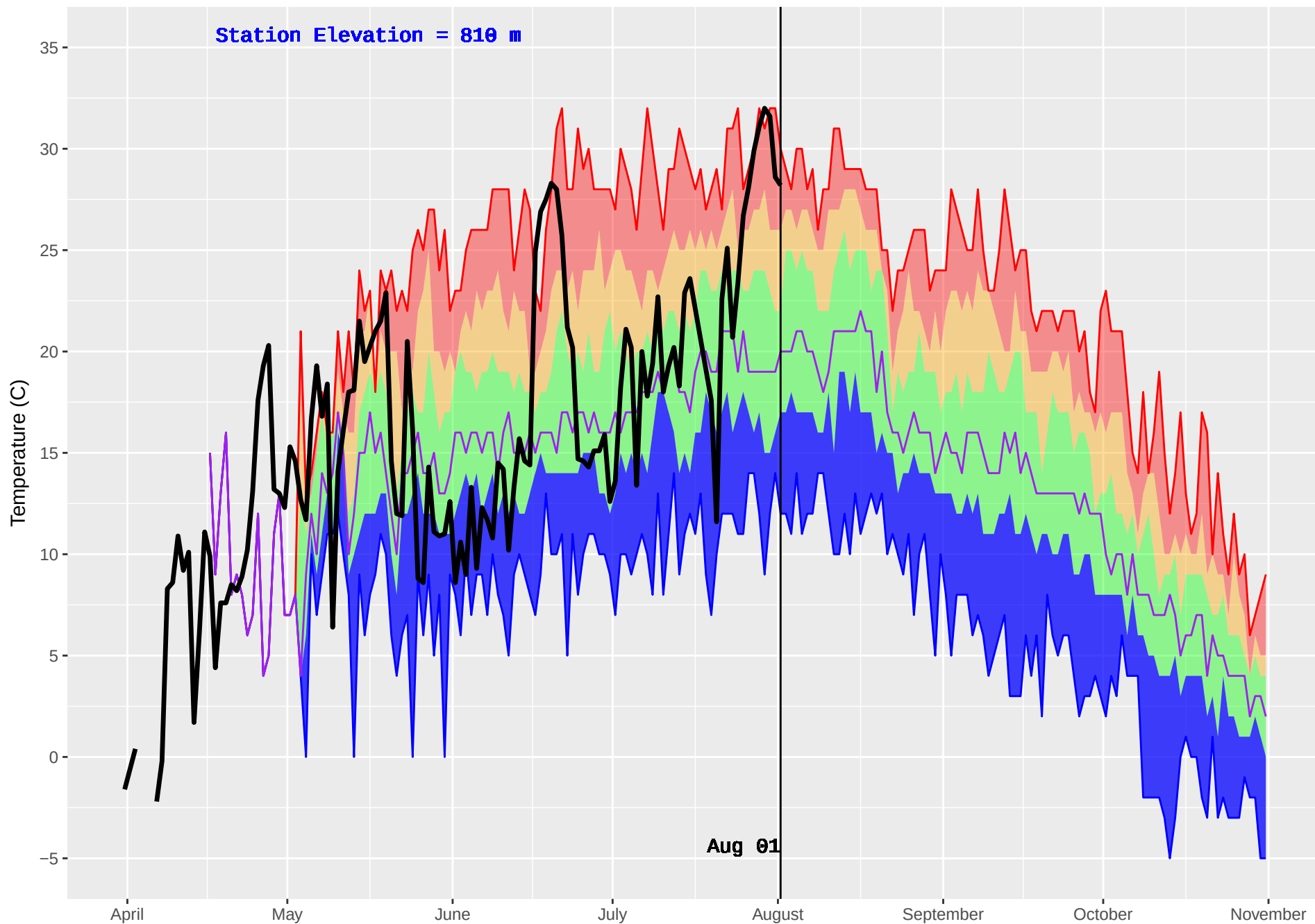
MCBRIDE LAKE (180) : Historical (1990–2016) and Current (2018) Daily Temperature
