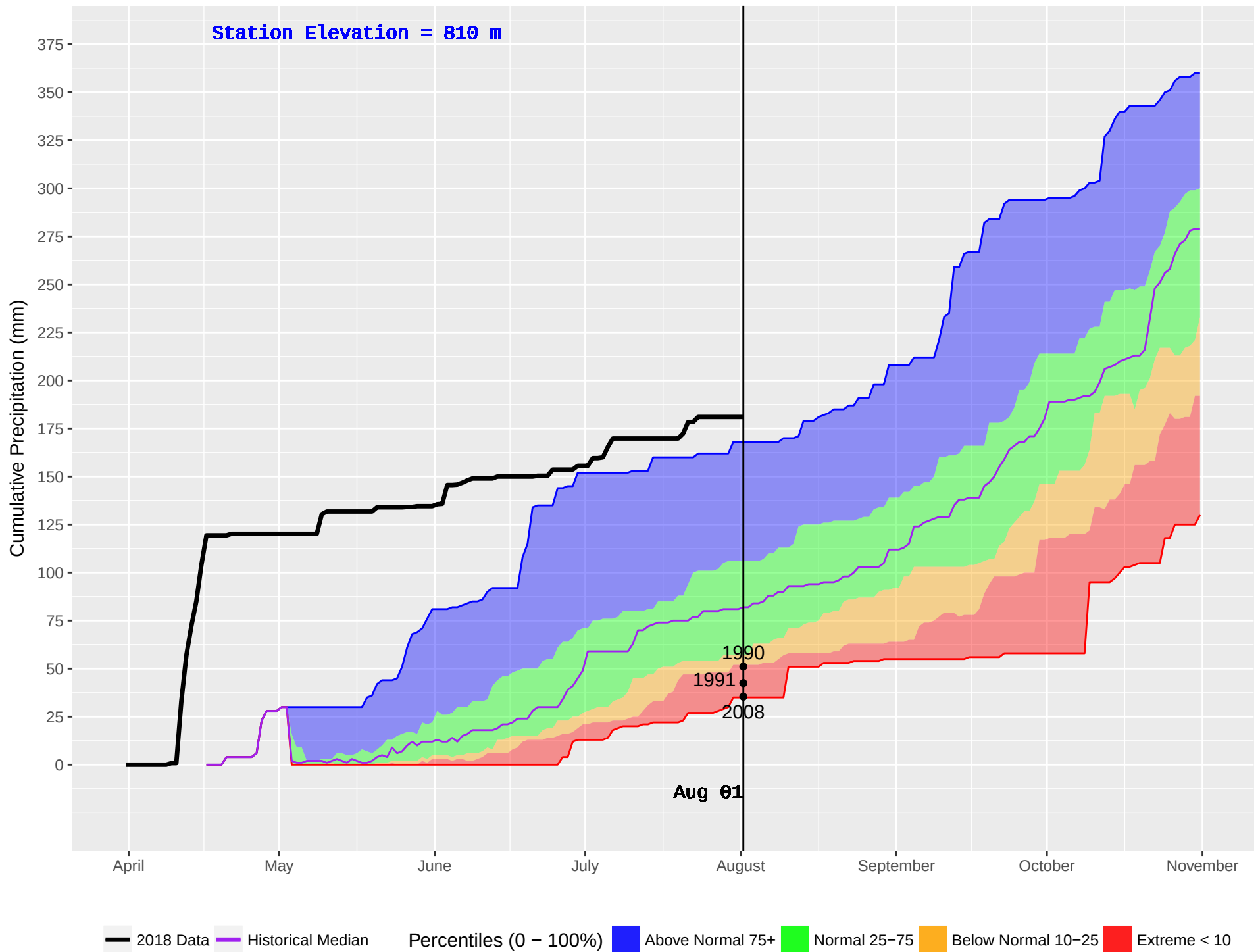
MCBRIDE LAKE (180) : Historical (1990–2016) and Current (2018) Daily Cumulative Precipitation
